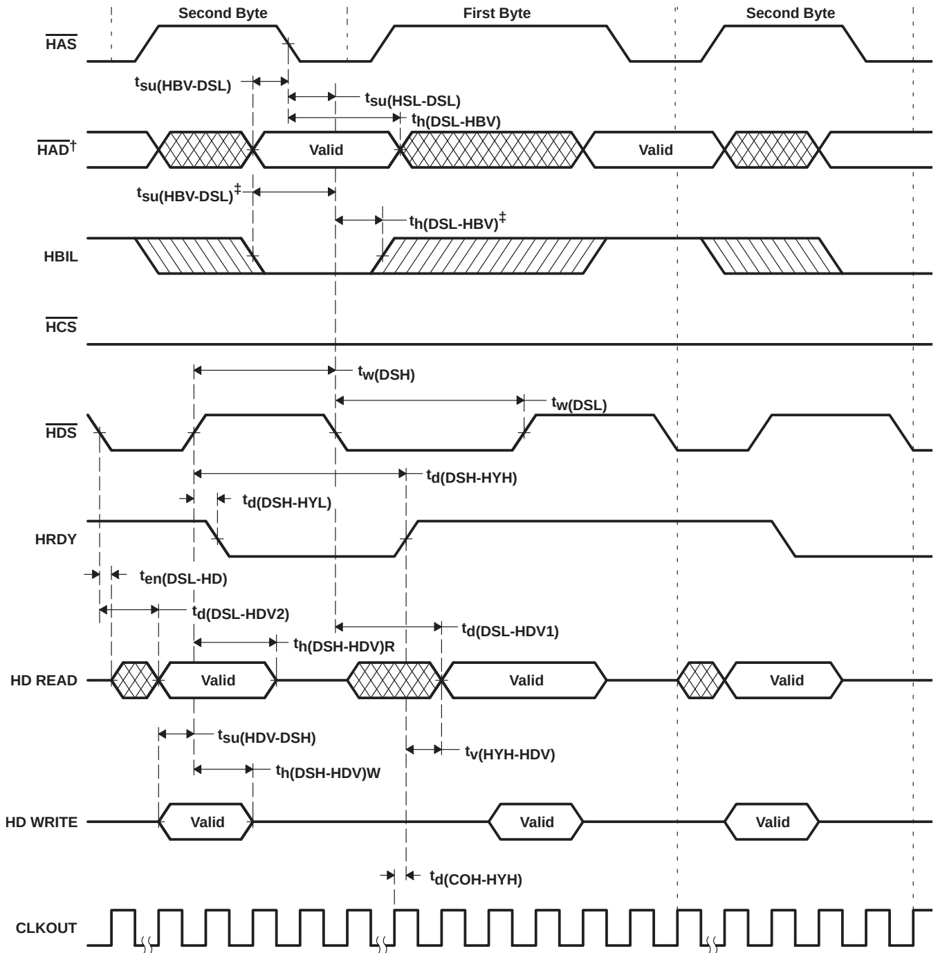
Figure 28. Using HDS to Control Accesses (HCS Always Low)
